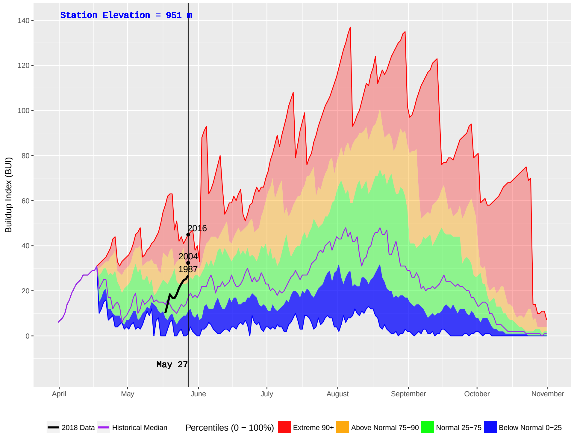
NORTH BABINE (173) : Historical (1986–2016) and Current (2018) Noon Buildup Index (BUI)
