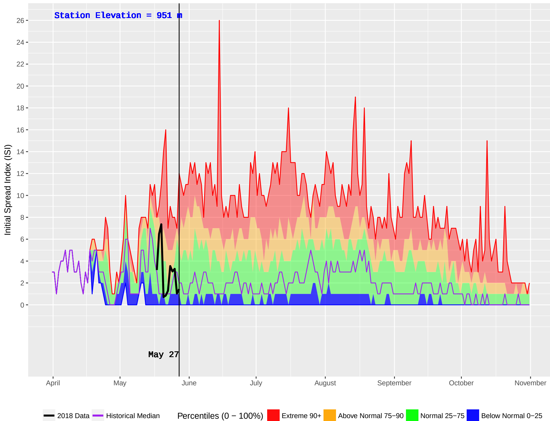
NORTH BABINE (173) : Historical (1986–2016) and Current (2018) Noon Initial Spread Index (ISI)
