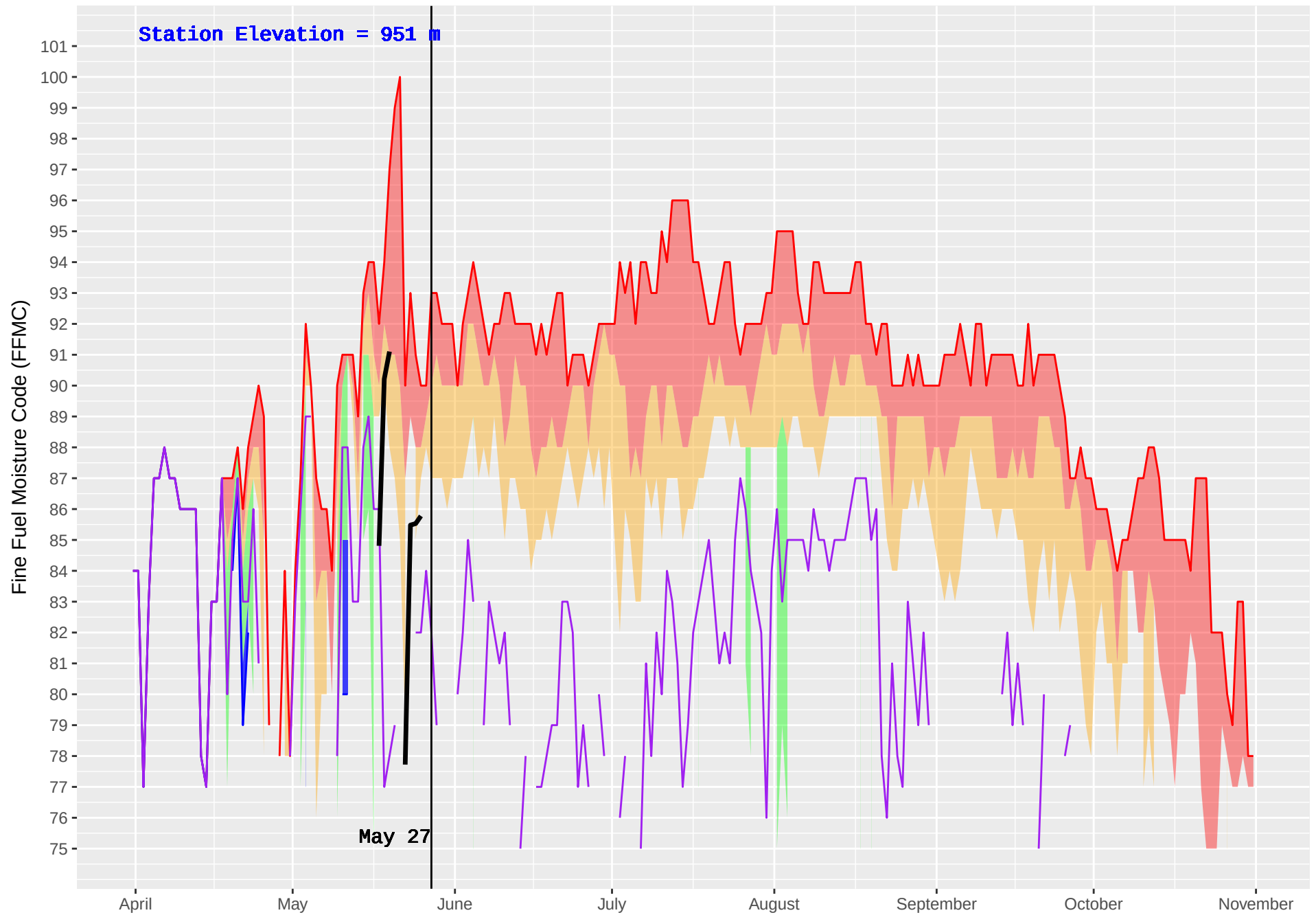
NORTH BABINE (173) : Historical (1986–2016) and Current (2018) Noon Fine Fuel Moisture Code (FFMC)
