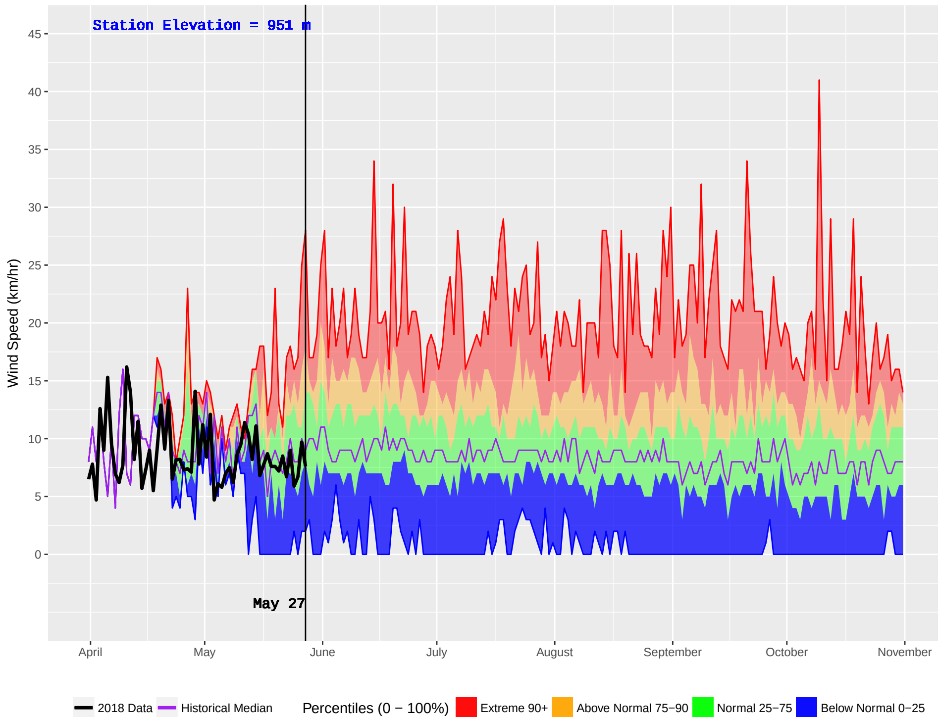
NORTH BABINE (173) : Historical (1986–2016) and Current (2018) Noon Wind Speed
