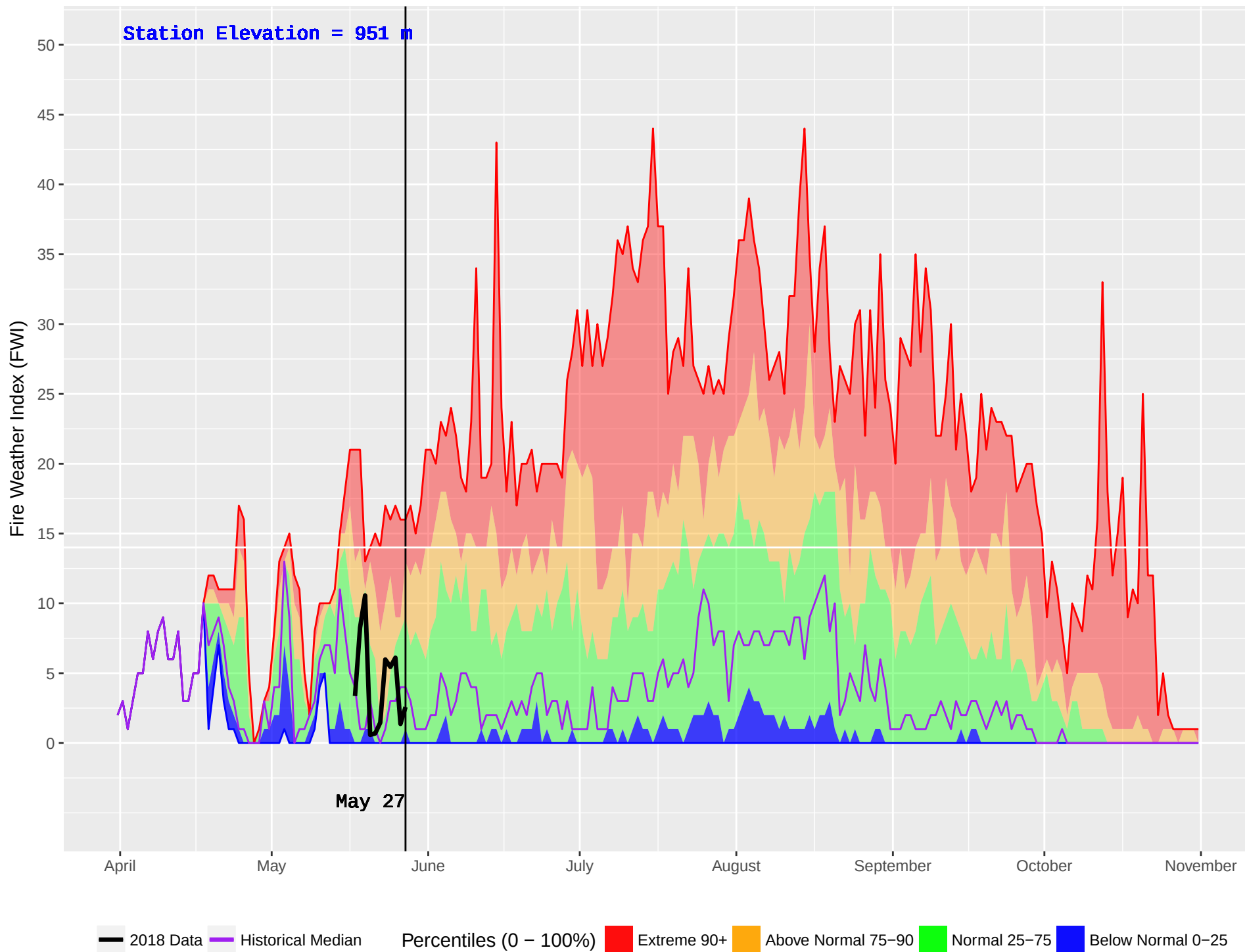
NORTH BABINE (173) : Historical (1986–2016) and Current (2018) Noon Fire Weather Index (FWI)
