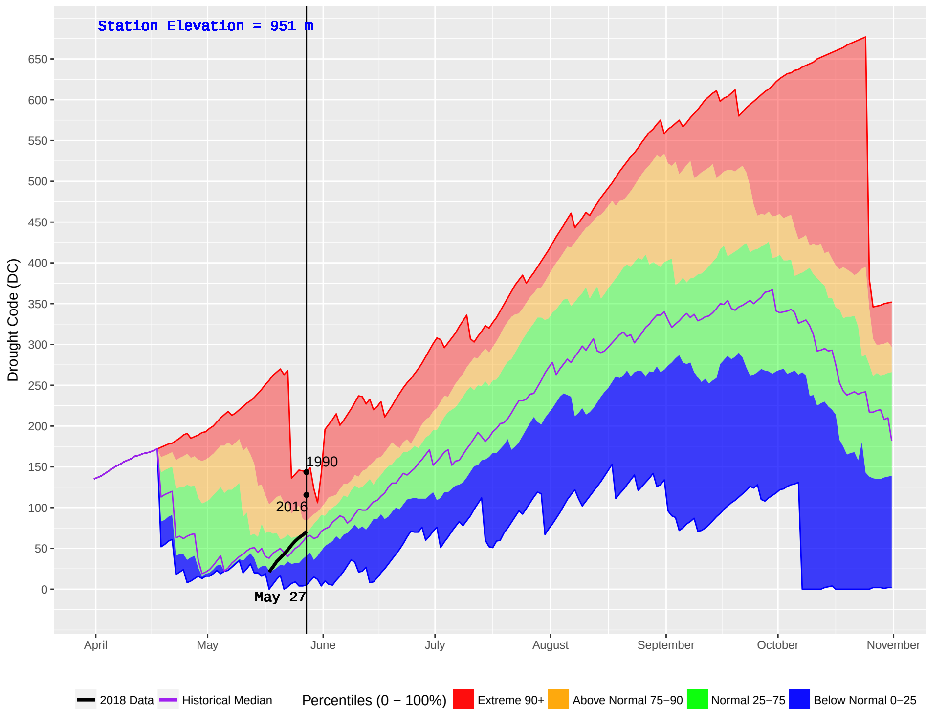
NORTH BABINE (173) : Historical (1986–2016) and Current (2018) Noon Drought Code (DC)
