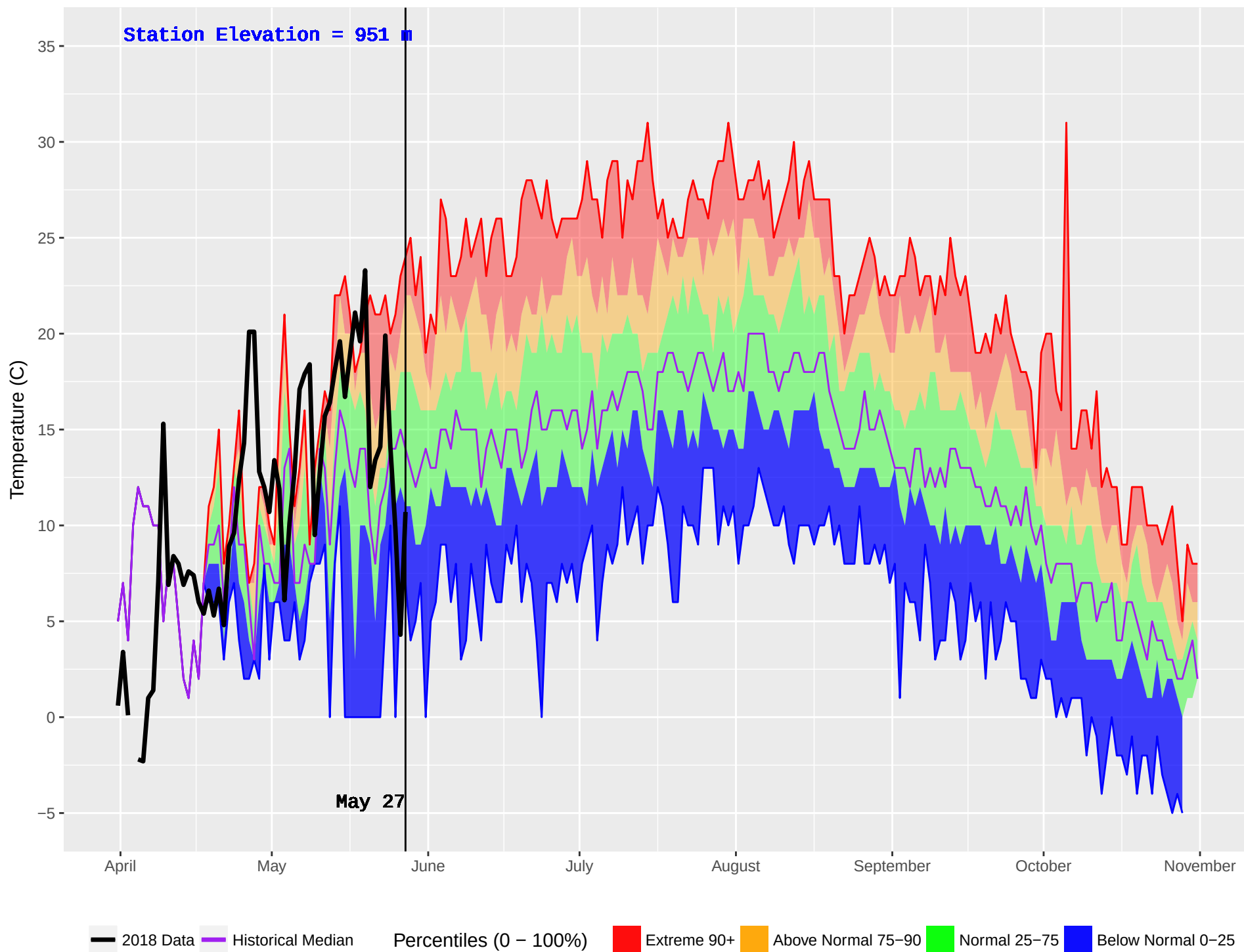
NORTH BABINE (173) : Historical (1986–2016) and Current (2018) Noon Temperature
