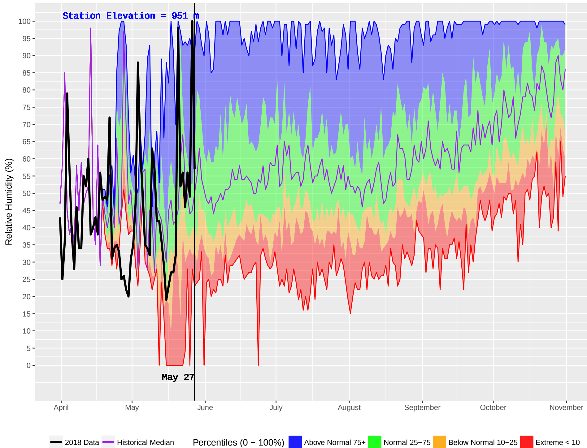
NORTH BABINE (173) : Historical (1986–2016) and Current (2018) Noon Relative Humidity
